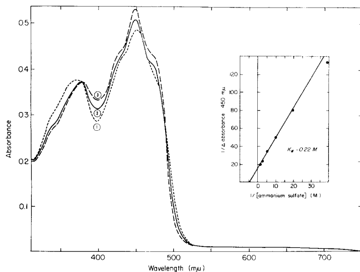
Fig. 5. Effect of (NH_4)_2SO_4 on the spectrum of glycolic acid oxidase. The enzyme was dissolved in 0.1 M sodium phosphate (pH 7.6). Curve 1, no additions; Curve 2, 0.10 M (NH_4)_2SO_4 ; Curve 3, 0.37 M (NH_4)_2SO_4 . The inset shows the Benesi-Hildebrand plot used to calculate K_d .
