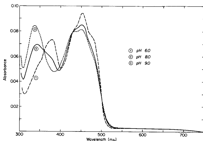
Fig. 8. pH titration of glycolic acid oxidase. The titration was performed in 0.09\text{ M} sodium phosphate.
