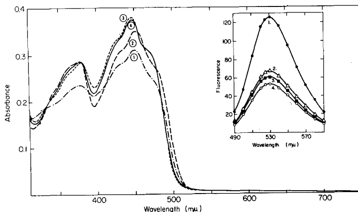
Fig. 6. Effect of heptanoate and oxalate on the spectrum of glycolic acid oxidase. The enzyme was dissolved in 0.1 M sodium phosphate (pH 7.6). Curve 1, no additions; Curve 2, 1.67 \cdot 10^{-2} M heptanoate; Curve 3, 9.91 \cdot 10^{-2} M oxalate; Curve 4, Curve 2 after addition of oxalate to a concentration of 9.91 \cdot 10^{-2} M. The inset shows the corresponding fluorescence emission spectra obtained by activating at 450 mμ.
