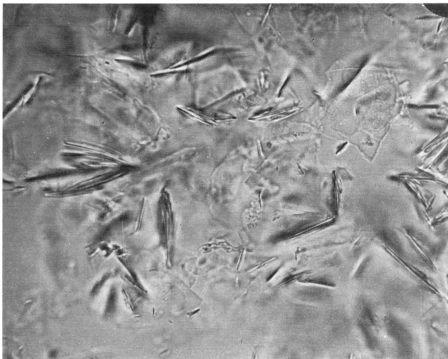
Fig. 1. Photomicrograph of glycolic acid oxidase crystals. The enzyme crystallized from a concentrated protein solution in 0.03 M sodium phosphate (pH 6.0). Magnification 500\times .
