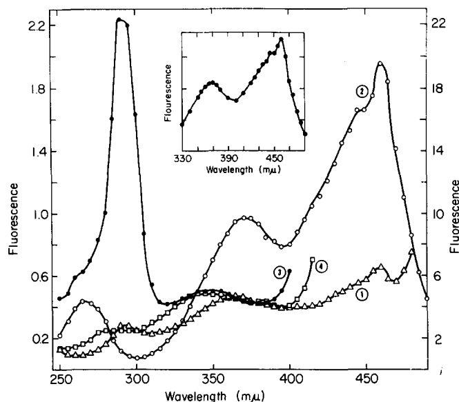
Fig. 12. Fluorescence activation spectra of green apoprotein before and after heating. Activation spectra obtained by measuring emission at 520\text{ m}\mu before and after heating are plotted in Curves 1 and 2, respectively. Curves 3 and 4 were obtained by measuring emission at 450\text{ m}\mu before and after heating, respectively. Emission intensity for Curves 1, 3 and 4 is represented by the left-hand scale whereas Curve 2 is plotted according to the scale on the right. Spectra were recorded in 0.1\text{ M} sodium phosphate ( \text{pH } 7.0 ) at 0-1^\circ . The inset shows the activation spectrum of an authentic sample of FMN.
